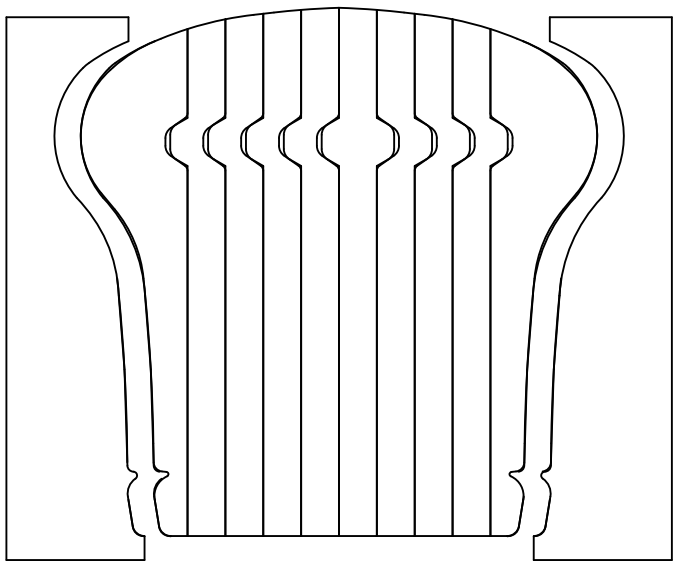
HWP4012B Handrail
