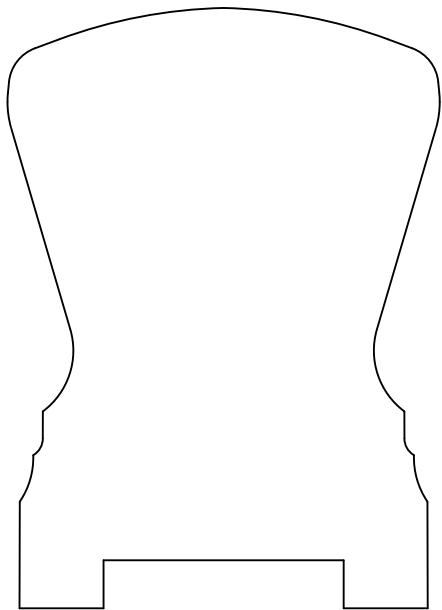
HWP4035 Handrail 3.125" x 2.250"
