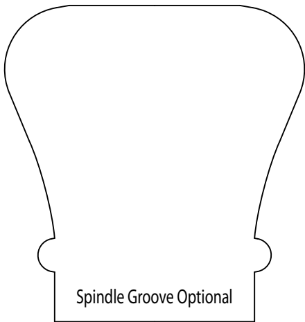
HWP4057 Handrail 2.375" X 2.250"
