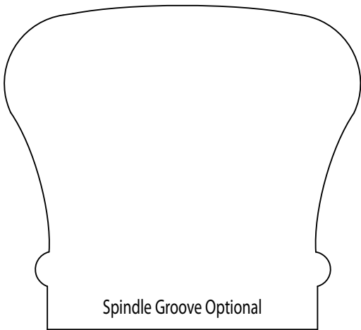
HWP4059 Handrail 2.375" x 2.625"
