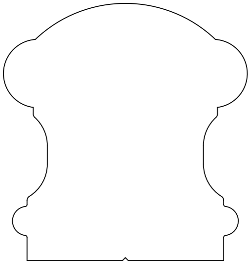
4072 Handrail 2.750" x 2.625"
