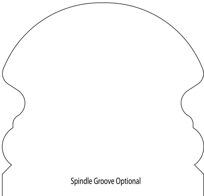
HWP4091 Handrail 3.250" x 3.750"
